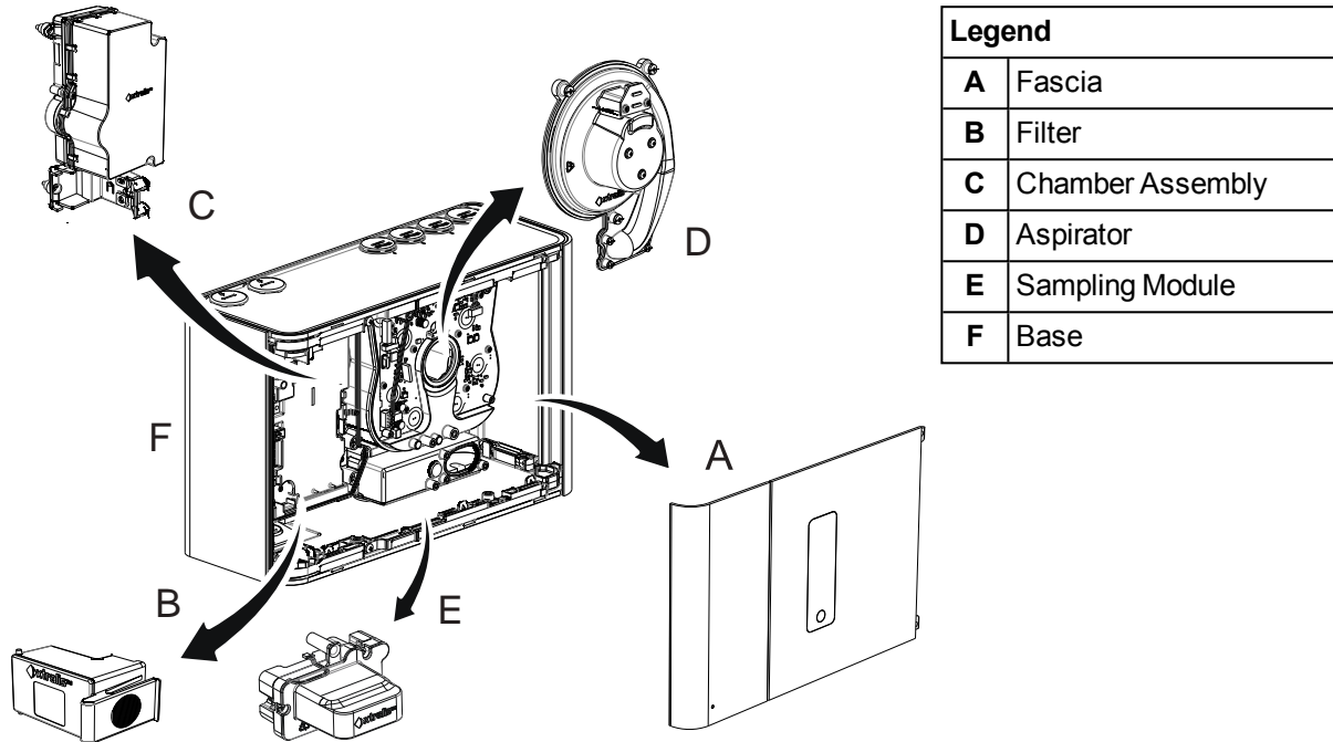
Figure 2-1: Detector components
